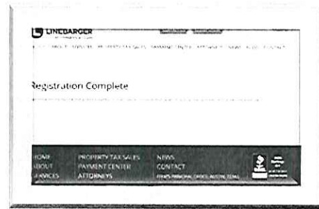
Figure 3 Confirmation Page
